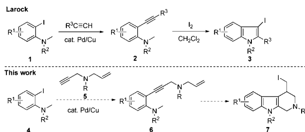
Scheme 1. Iodine-Mediated Cascade Cyclization of Enynes to Iodinated Tetrahydro- \beta -carbolines
