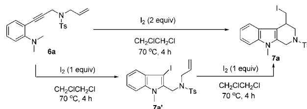
Scheme 2. Control Experiment
