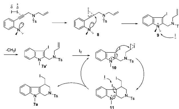
Scheme 3. Proposed Mechanism
