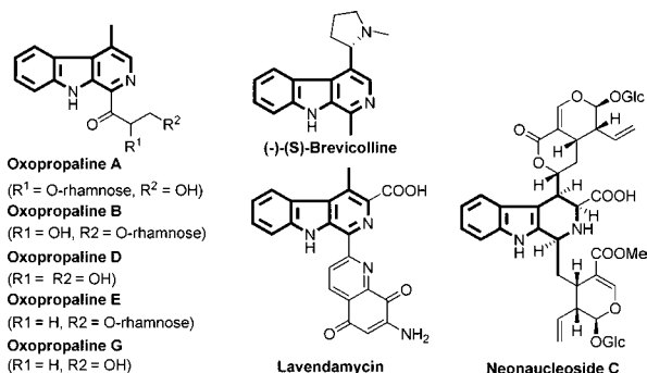
Figure 1. Selected examples of 4-substituted carboline alkaloids and tetrahydrocarboline alkaloids.
